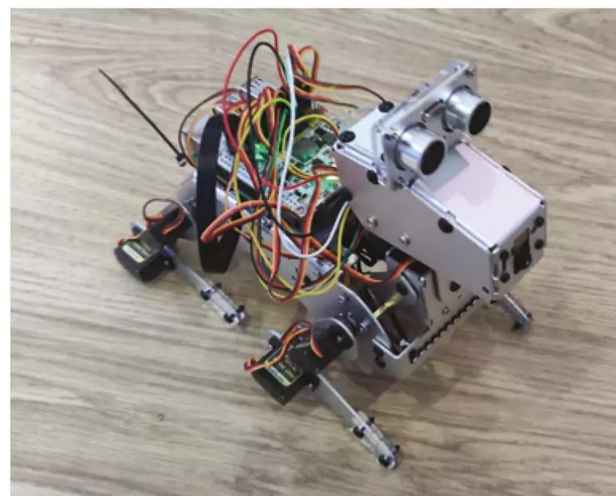
▲ You'll end up with spaghetti wiring into the Robot HAT, but can use the supplied spiral binding to tidy it up a bit
