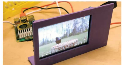
▲ Raspberry Pi Zero and an Elecrow touchscreen form the project's basis, all wrapped in a custom enclosure
